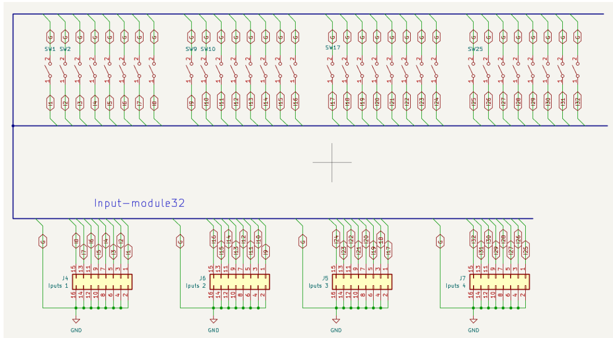
Figure 4: Direct switch wiring diagram
