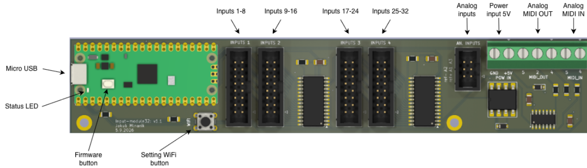
Figure 3: Overall layout of the board
