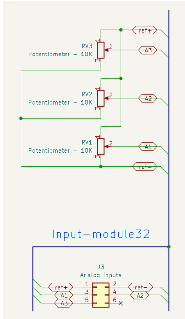
Figure 5: Potentiometer wiring for analog inputs
